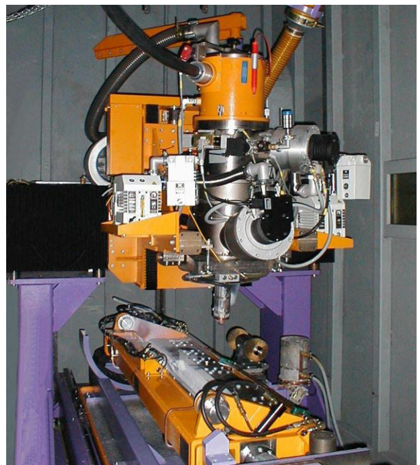
EB generator with portal and clamping device
